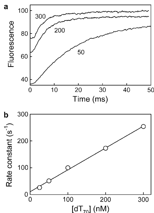
FIGURE 4 Association kinetics of DCC-SSB with dT 70 . (a) A 5-nM DCC-SSB tetramer was mixed with various concentrations of dT 70 and fluorescence intensity followed with time in a stopped-flow apparatus. Conditions were as in Table 1, except that measurements were performed at 25°C. Typical individual traces at nanomolar concentrations of dT 70 are shown. Traces were normalized to finish at 100% and offset by 5% from each other. The fast traces have diminished amplitude, mainly due to loss of signal during the dead time of the instrument (~2 ms). Individual fluorescence traces fitted single exponentials well and the rate increased with DNA concentration. (b) Dependence of rate on concentration of DNA. Data shown are the averages of typically three traces from each of two separate experiments.
